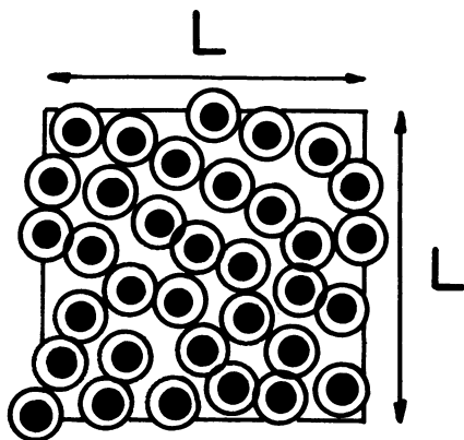
FIGURE 3 The black disks indicate the cross-section of fibrils with a radius R_F = 13 nm, inside a box with side-length L = 0.25 \mu m. The position and the size ( R_F = 13 nm) of the fibrils have been taken from a portion of Fig. 3 e of reference 11. The open circles around each disk have a radius of R_C = 18.25 nm.
